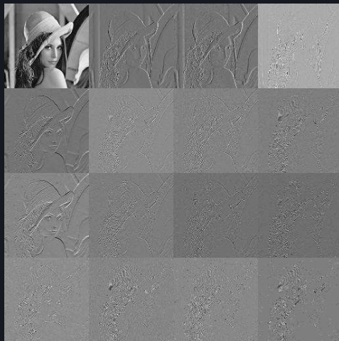
Proposed method, 5910 bytes (0.167 bit/px), RMSE: 17.27/6.51, PSNR: 23.38 dB/31.86 dB
